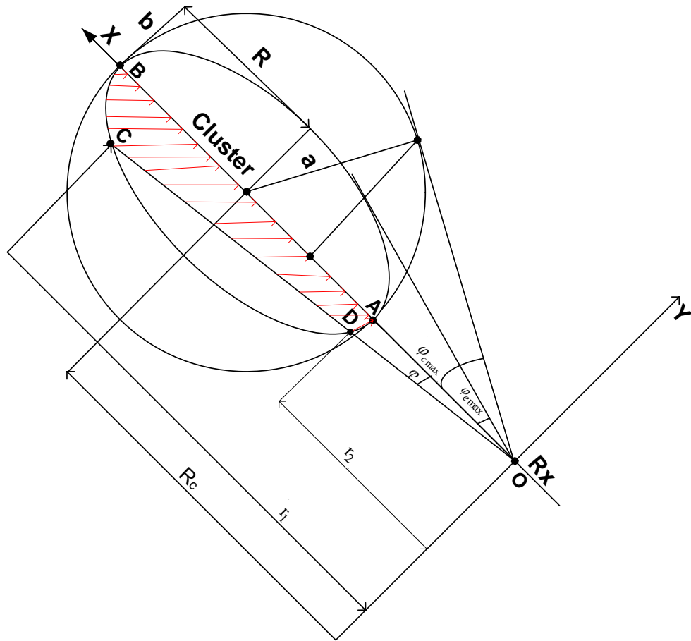
Figure 5.1 Geometry of the model for the calculation of the PDF of DOA.
