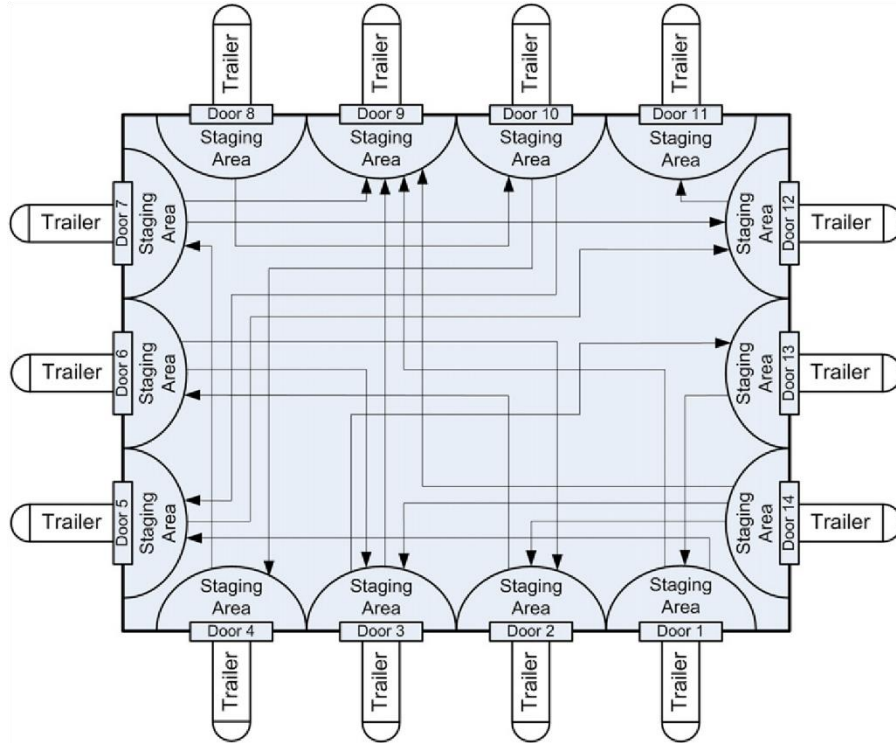
Figure 1: Structure and operation of the proposed cross-docking model.
