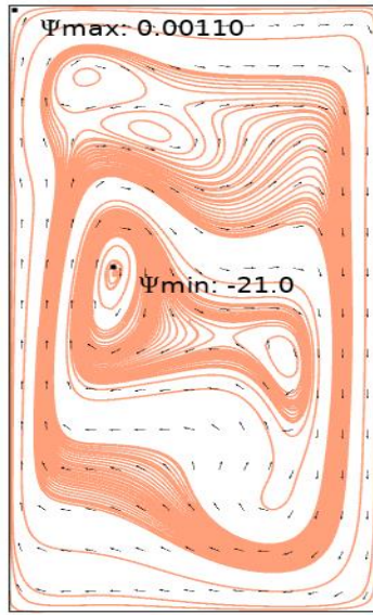
(b) Ra = 10^7
