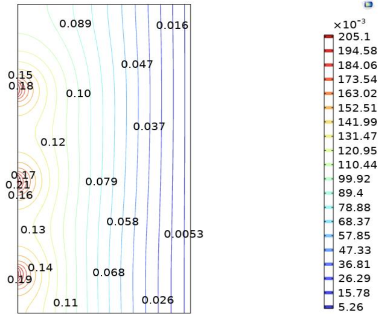
(b) Ra = 10^7
