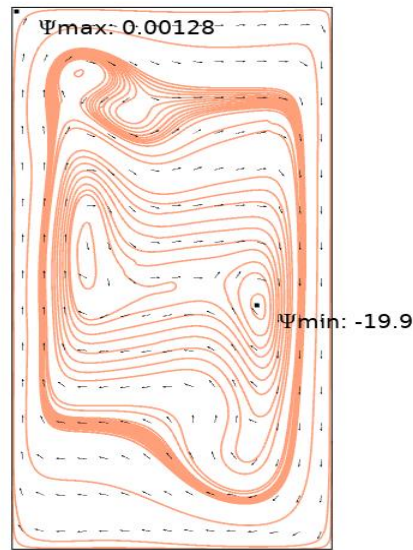
(b) Ra = 10^7
