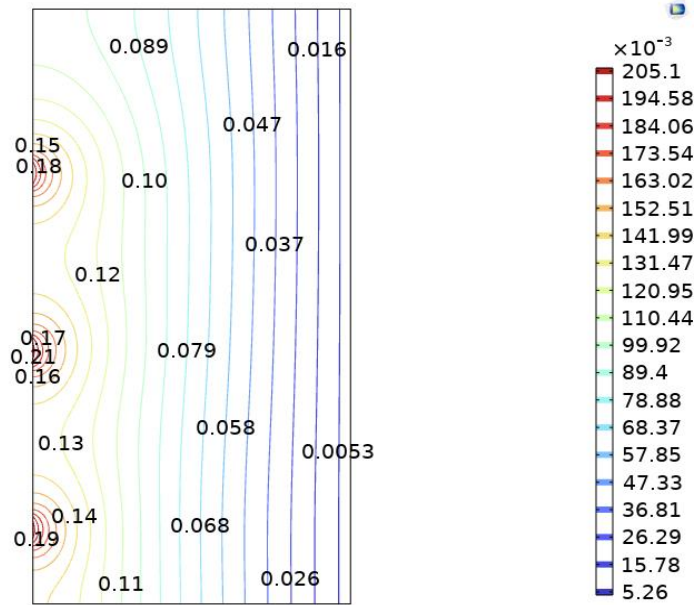
(a) Ra = 10^3
